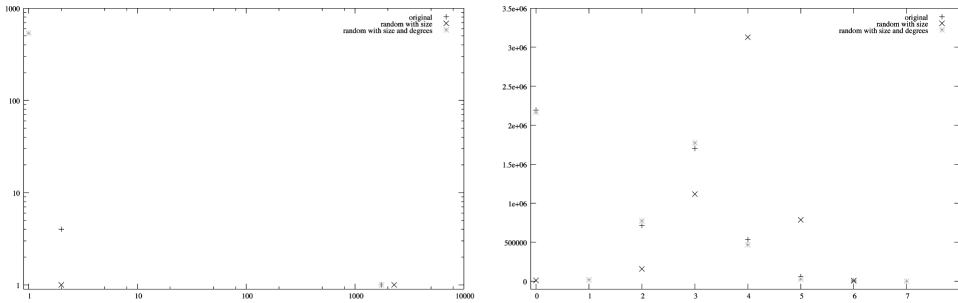
FIG 3. – Left: the connected component size distribution. Right: the distribution of distances between pairs of nodes. Each plot is given for both the original interaction network, for a typical random graph of same size, and for a typical random graph with the same size and degree distribution.
