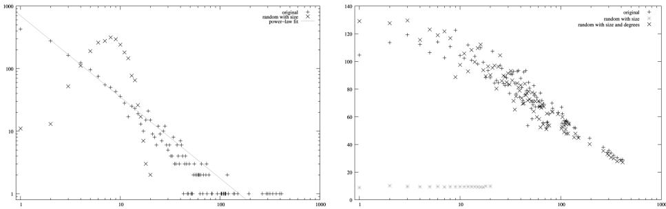
FIG 1. – Left: the degree distribution of the original interaction network, fitted by a power law of exponent \alpha = 1.3 , and the one of a typical random graph of same size. Right: the degree correlations, i.e. the average degree of neighbors of nodes of degree i as a function of i , for both the original interaction network, for a typical random graph of same size, and for a typical random graph with the same size and degree distribution.
