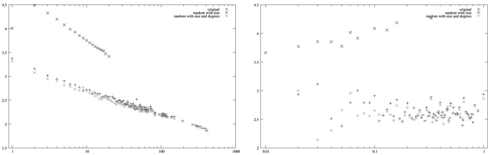
FIG 4. – Left: the correlations between centrality and degree, i.e. for all i the average distance of nodes of degree i to all others. Right: the correlations between centrality and clustering, i.e. for all \frac{i}{100} the average distance of nodes of clustering between \frac{i-0.5}{100} and \frac{i+0.5}{100} to all others. Each plot is given for both the original interaction network, for a typical random graph of same size, and for a typical random graph with the same size and degree distribution.
